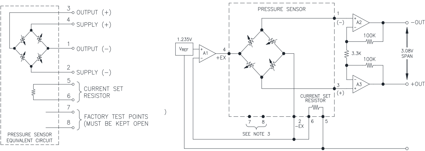
APPLICATION SCHEMATIC
